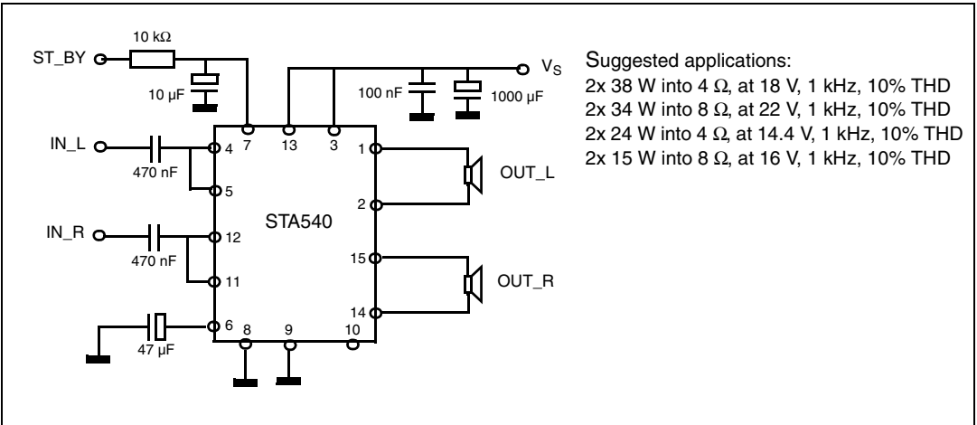
Figure 5. Dual bridge
