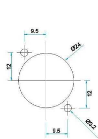
Installation hole figure
