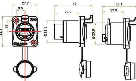
S socket (dimensions figure)
