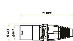
Plug (dimensions figure)
